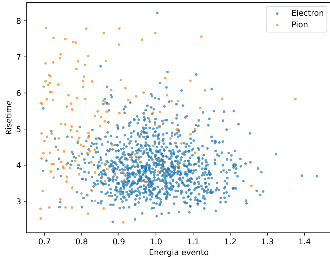
Scatter plot e/pi (cutted) 1.0GeV
