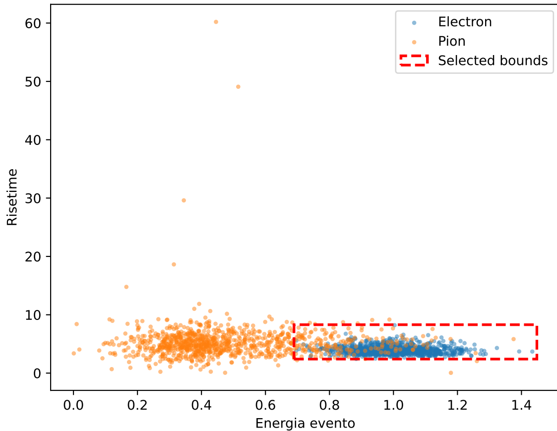
Scatter plot e/pi (all) 1.0GeV
